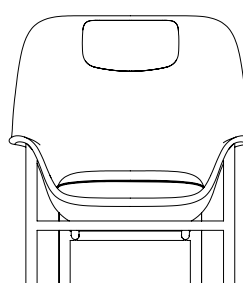
Drape Lounge Chair high w. headrest wood legs H: 116,5 x L: 82,5 x D: 82,5 x SH: 43 cm
