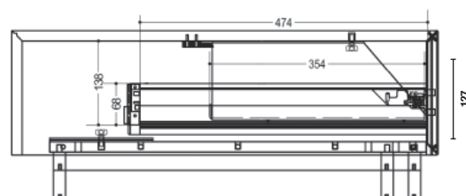
DRAWER, videorecorder/DVD rack H 12.7
